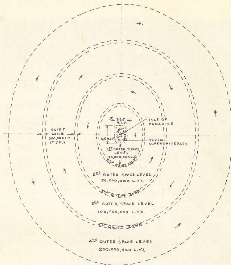
LOGARITHMIC PLAN VIEW OF THE GRAND UNIVERSE
